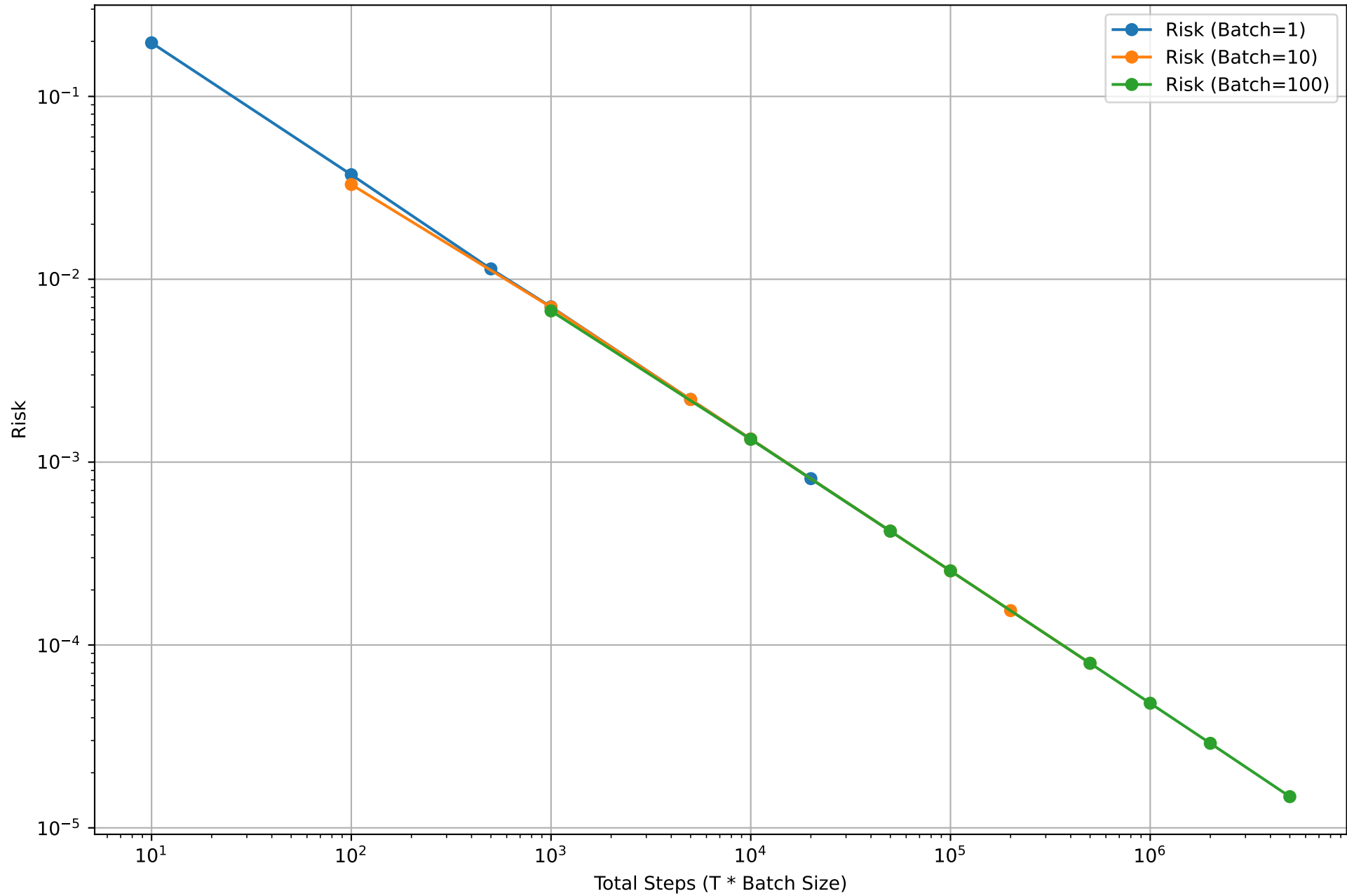
Slock Risk for Different Batch Sizes; \alpha=1.9 . optiized eta_star for each T
